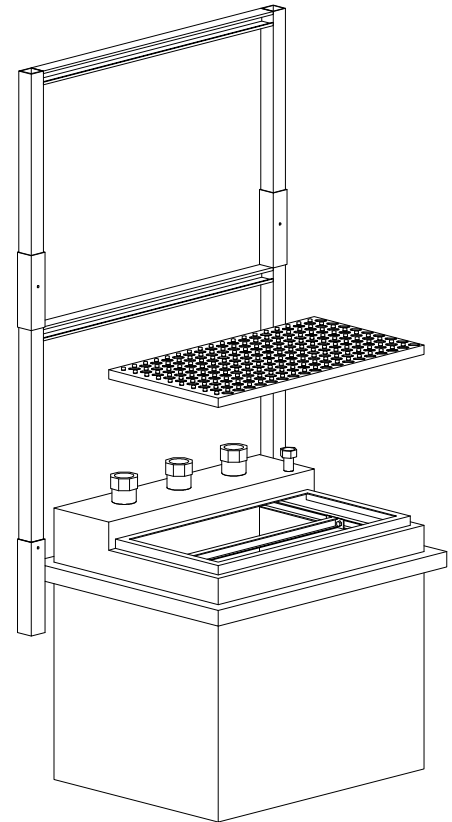
3D VIEW
