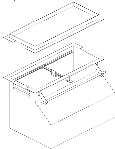
3D VIEW
