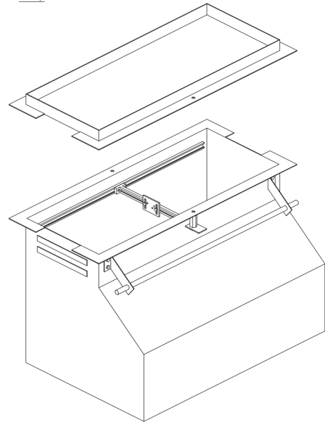
3D VIEW
